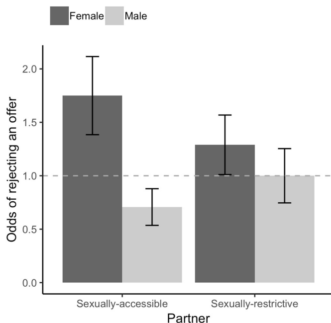
Fig. 3. Odds for accept-reject rates in the Ultimatum Game (UG), as a function of context and participant sex. Note. Error bars standard error. Dashed line reflects the point of indifference between accept and reject, OR = 1.
