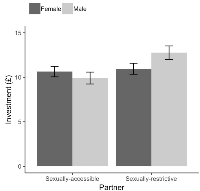
Fig. 2. Mean investment in the Trust Game (TG) as a function of context and participant sex. Note. Error bars denote standard error.
